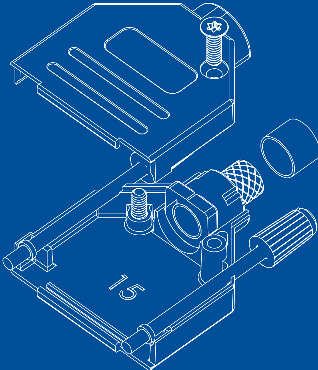
LINECARD EMI/RFI SHIELDED D-SUB BACKSHELLS
